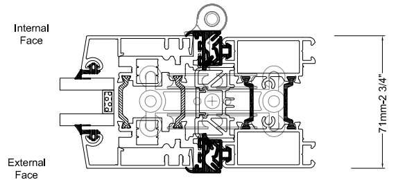
Section 4: Jamb with Roller Assembly
