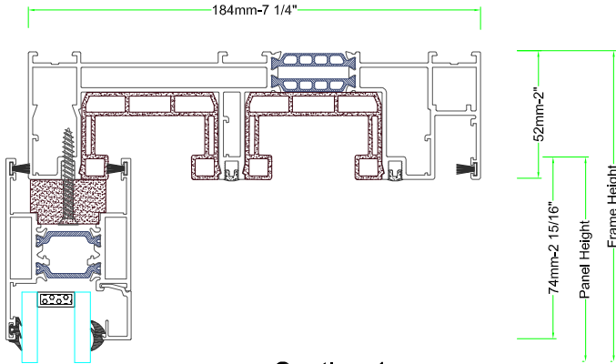
Section 1: Fixed Panel
