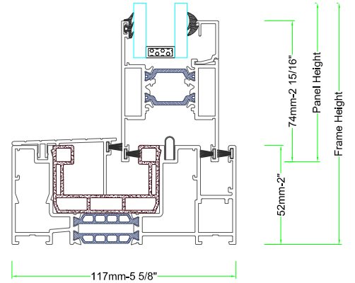
Section 5: Jamb with Sliding Panel
