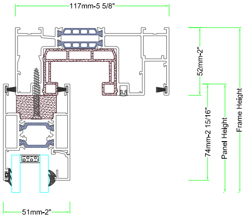
Section 1: Fixed Panel
