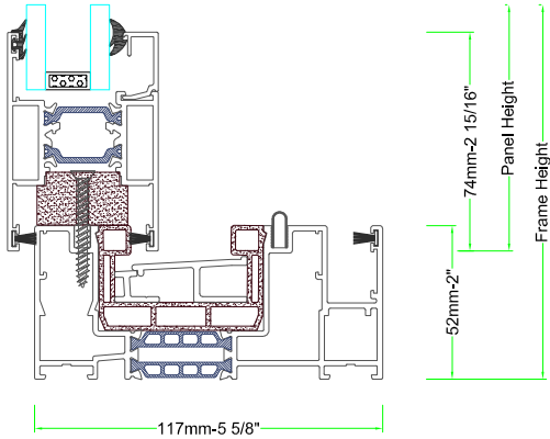
Section 3: Jamb with Fixed Panel
